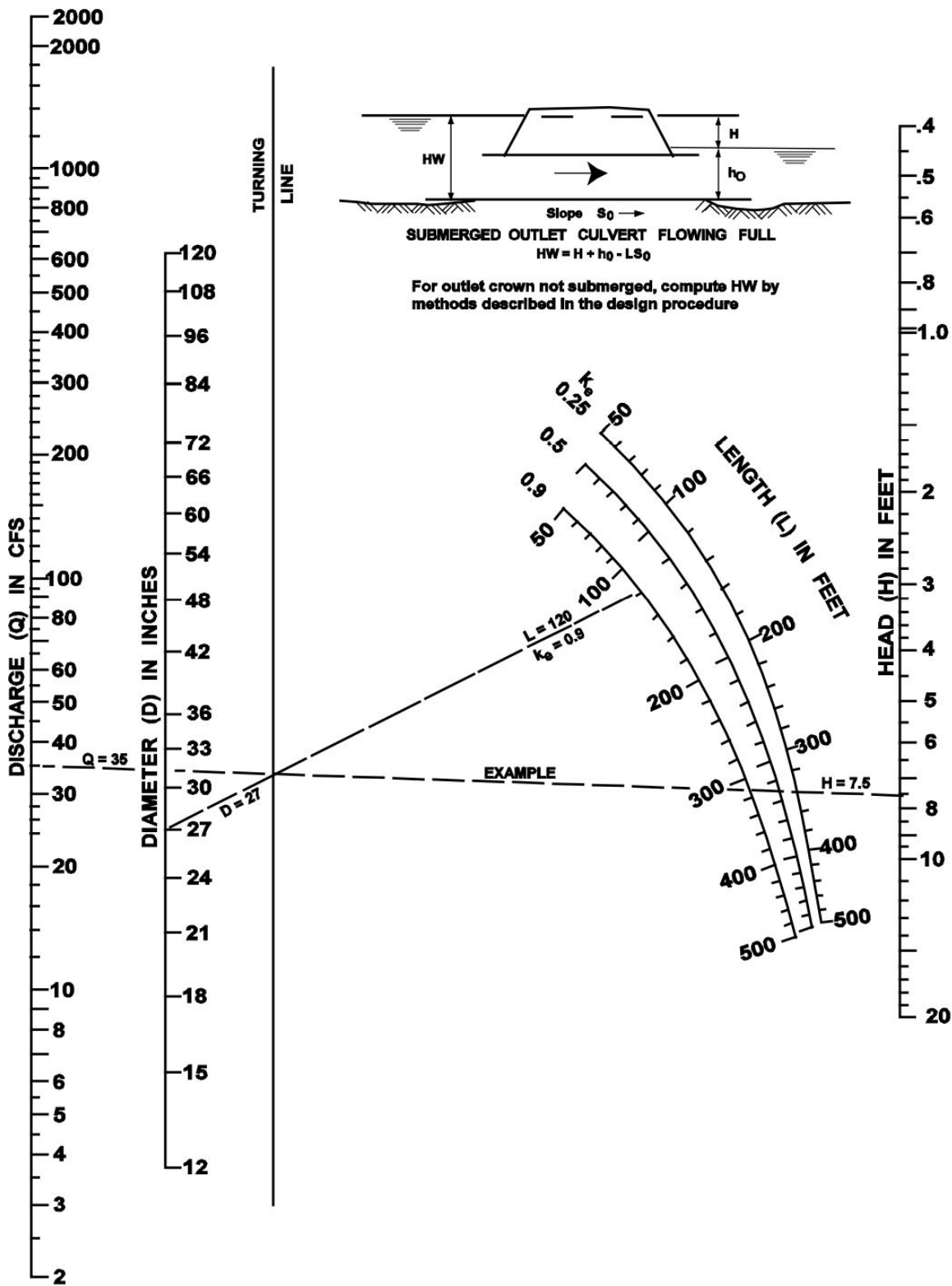
Figure F.11 Head for Culverts (Pipe with n=0.024 ) Flowing Full with Outlet Control
