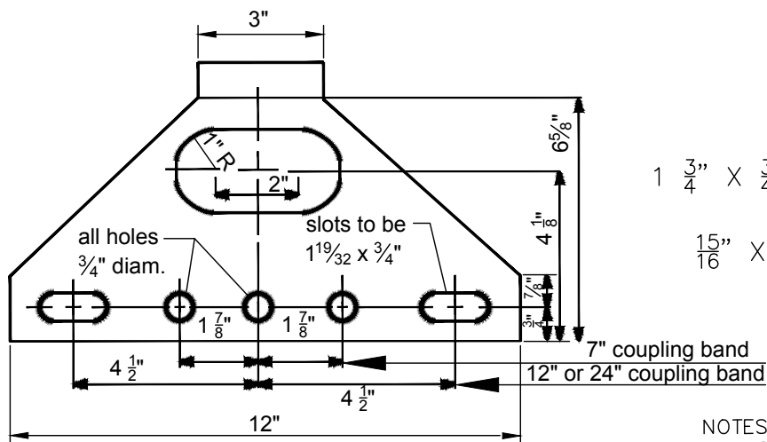
Plate Detail
