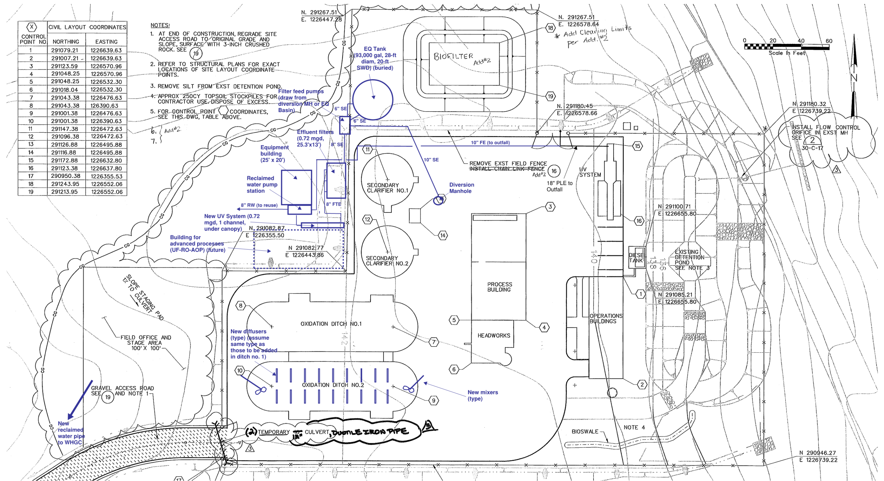
Figure 8-2. Preliminary site layout of recycled water facilities
