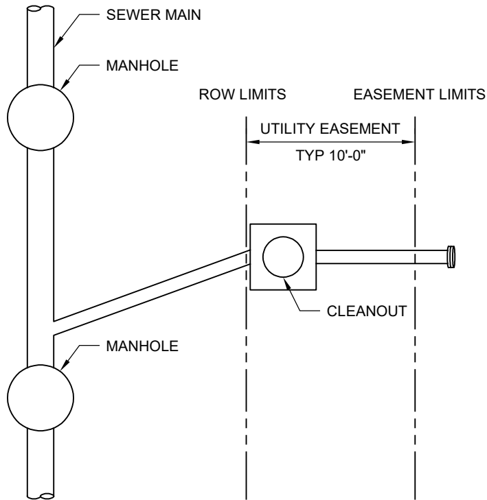
PLAN NTS
