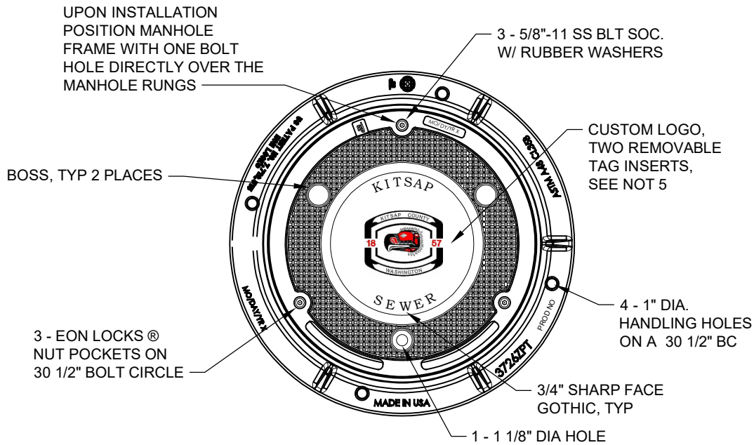
PLAN NTS
