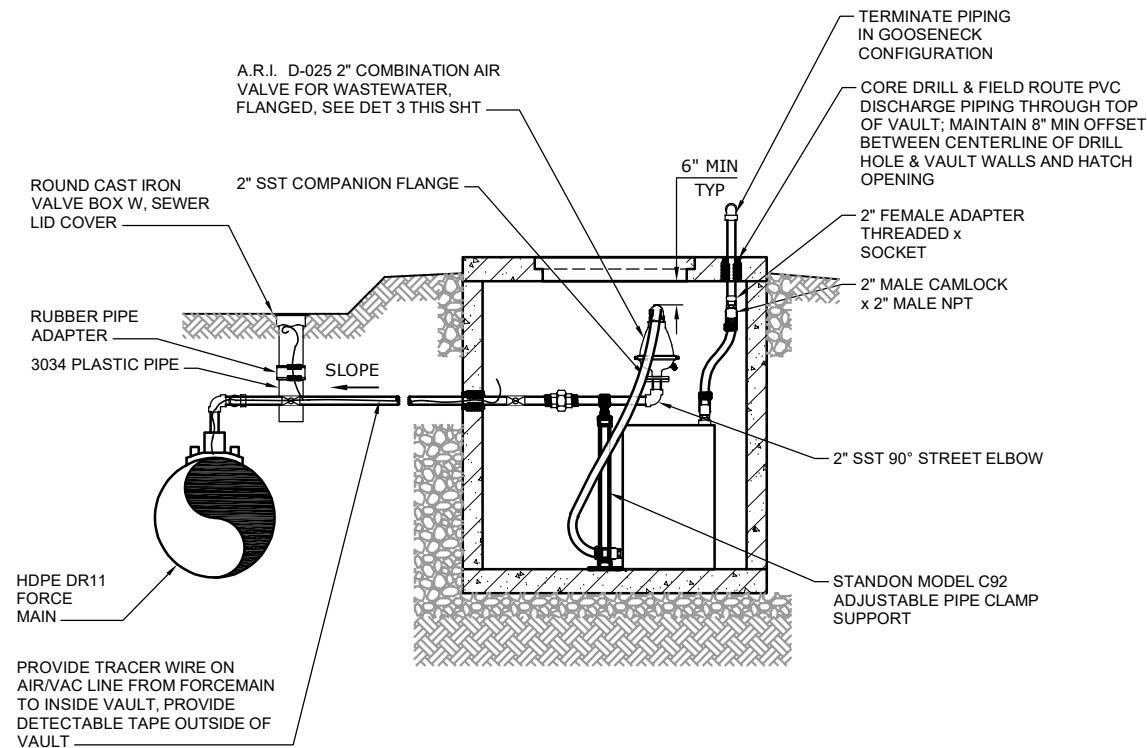
SECTION
