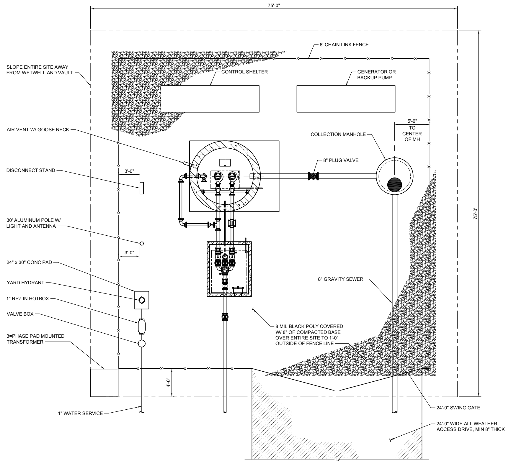
PUMP STATION SITE LAYOUT PLAN
