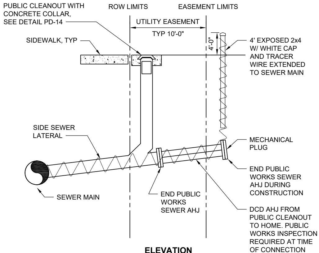
ELEVATION NTS
