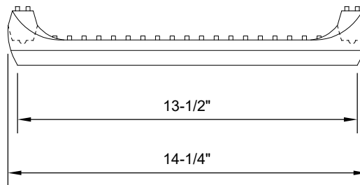
ELEVATION NTS
