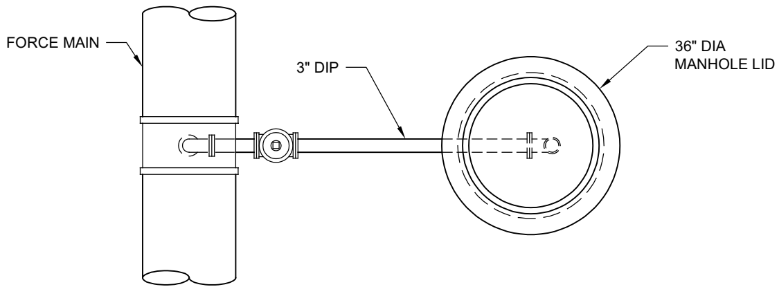
PLAN NTS
