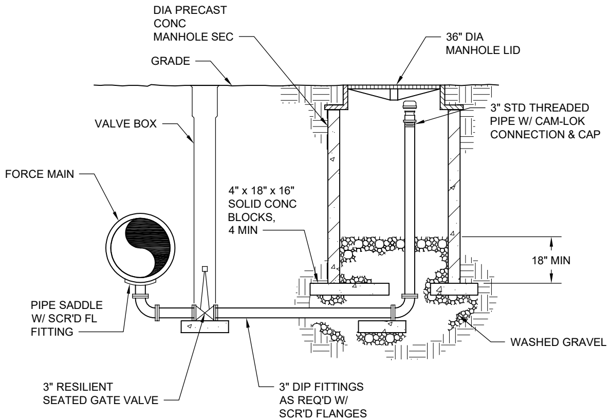
ELEVATION NTS
