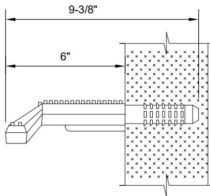
SECTION NTS
