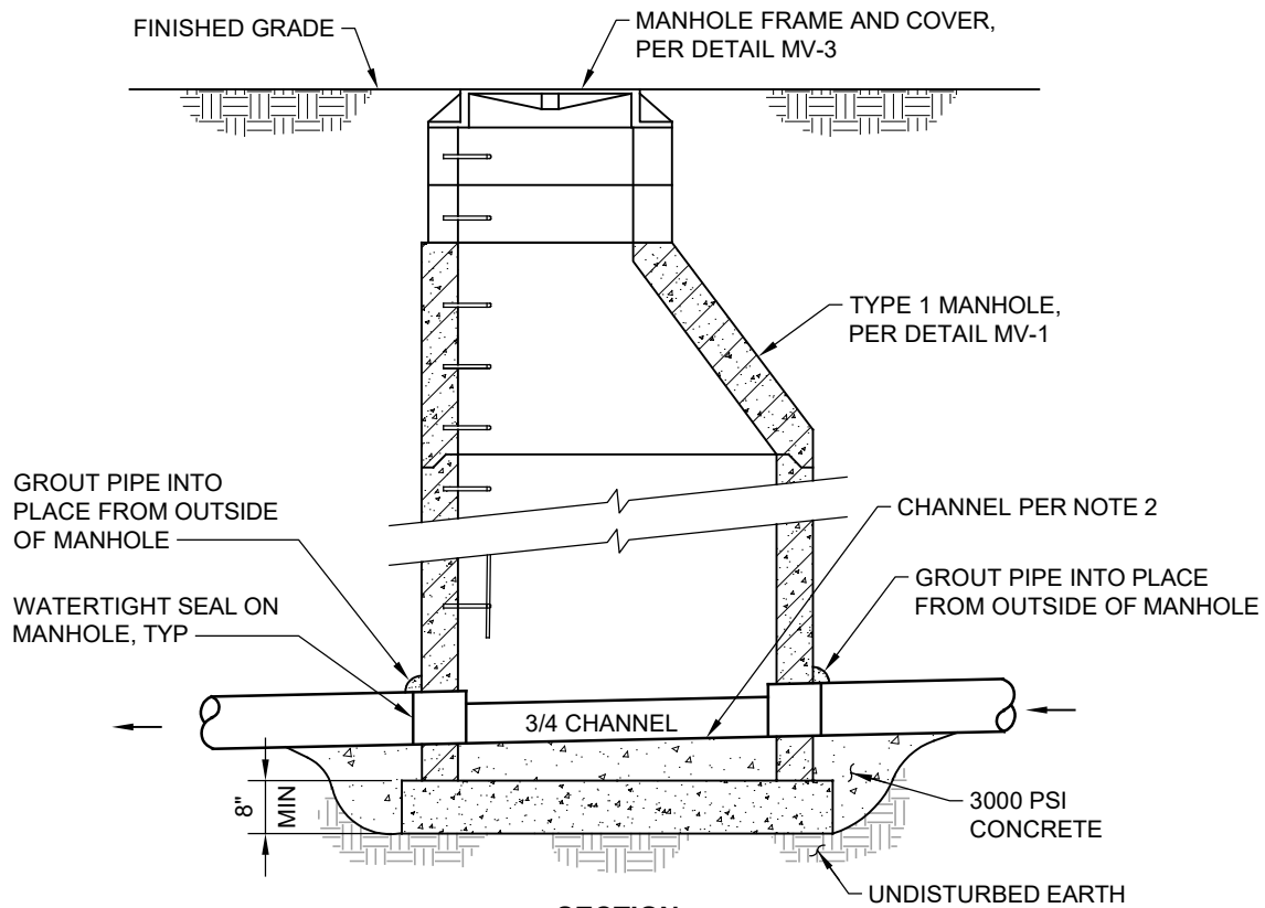
SECTION NTS
