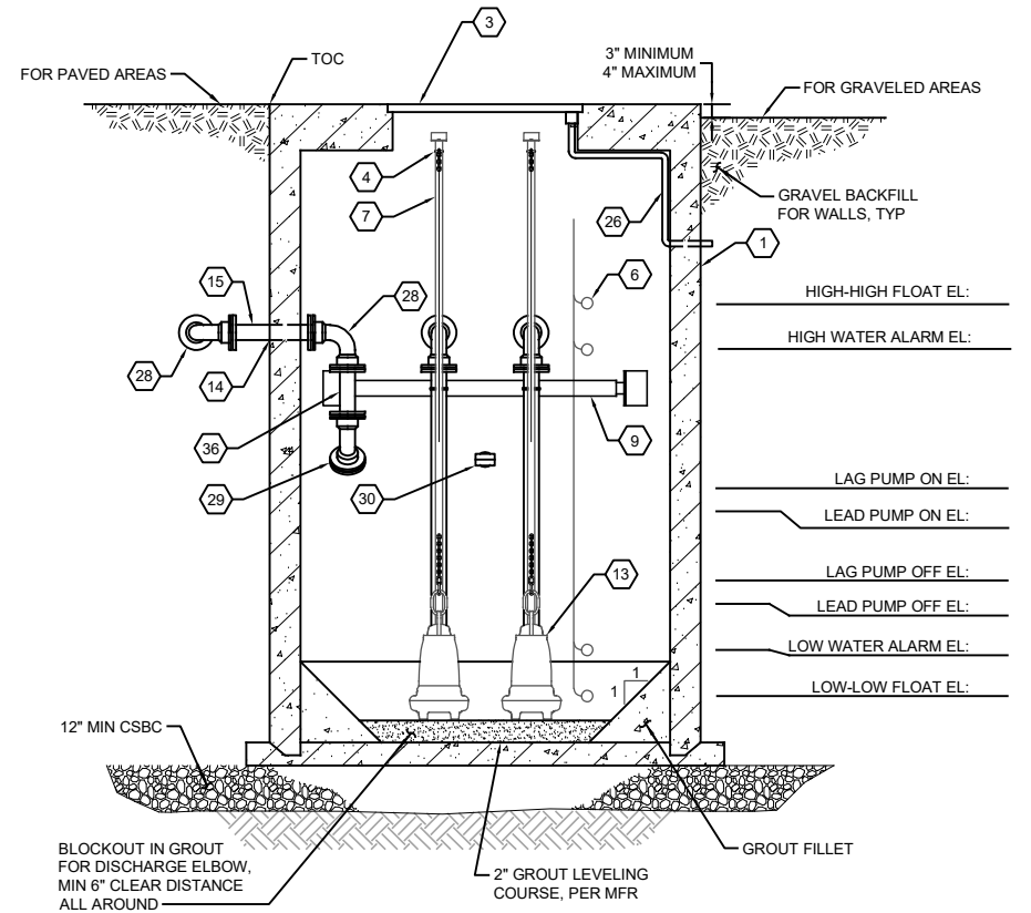
PUMP STATION SECTION
