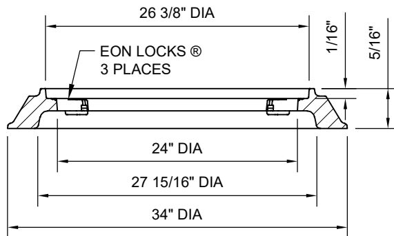
SECTION VIEW
