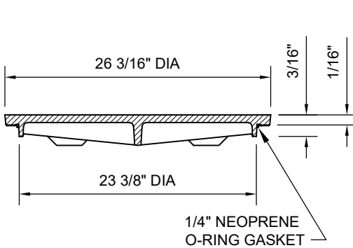
COVER SECTION
