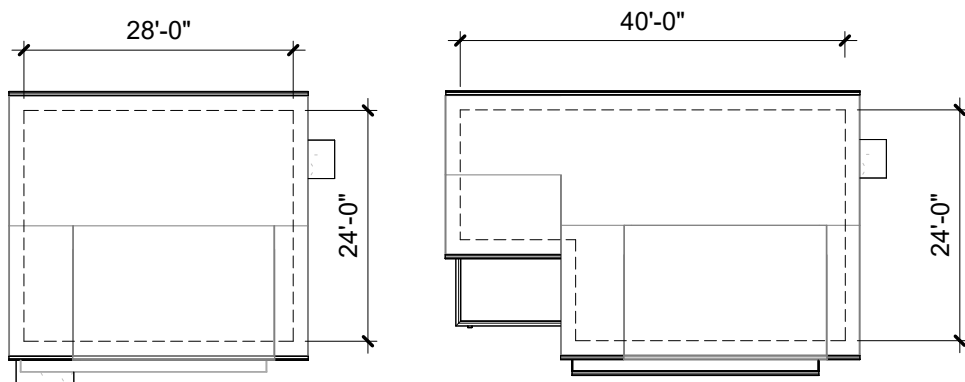
SITE PLANS @ 1:20
