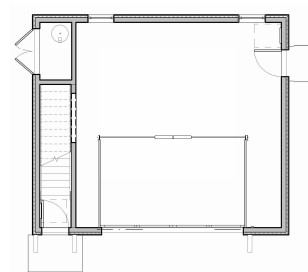
FIRST FLOOR
