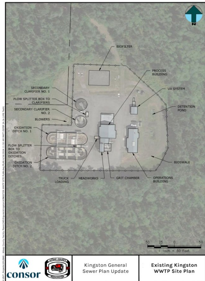
Figure 1. Existing Kingston WWTP Site Plan
